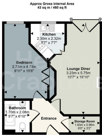
Floorplan
